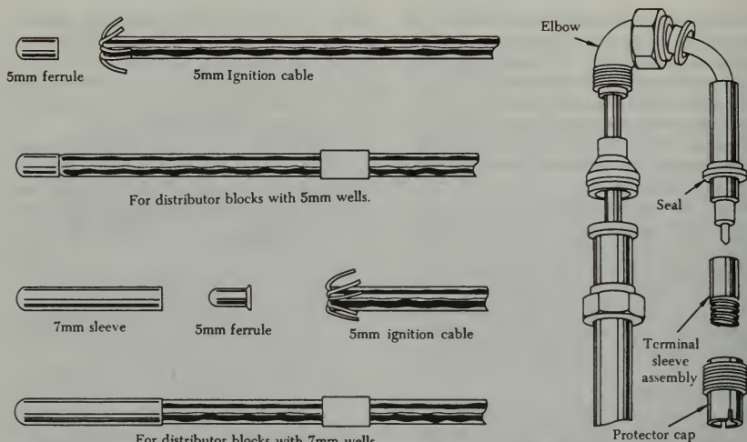
FIGURE 4-50. Replacement procedure for ignition lead terminals.
